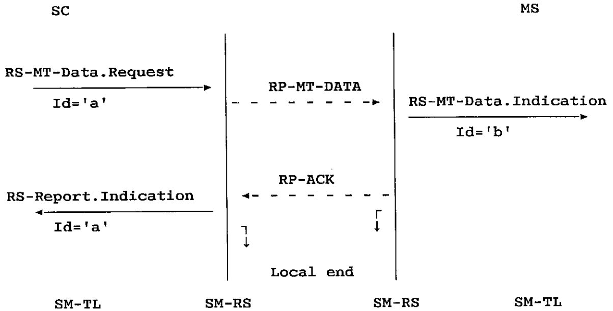
Figure 03.40/10a. Relationship between SM-RS primitives and relay layer protocol elements in the SM MT case.
