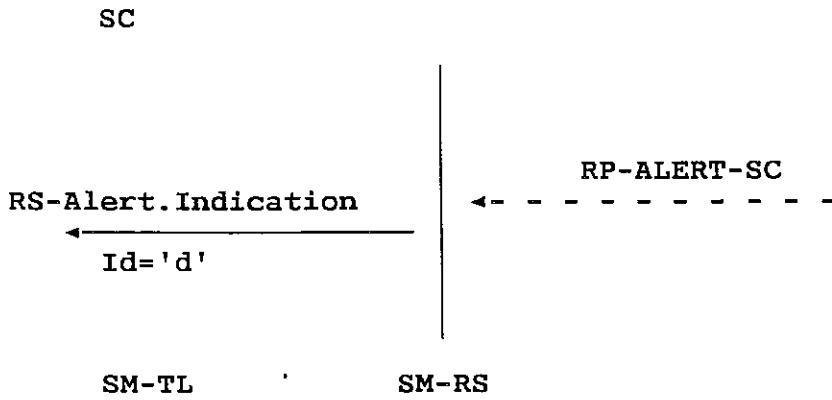
Figure 03.40/11. Relationship between SM-RS primitives and relay layer protocol elements in the Alert case.
