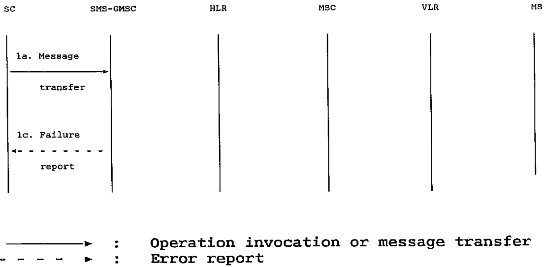
Figure 03.40/15 b). Short message transfer attempt failing due to error at the SMS-GMSC.
