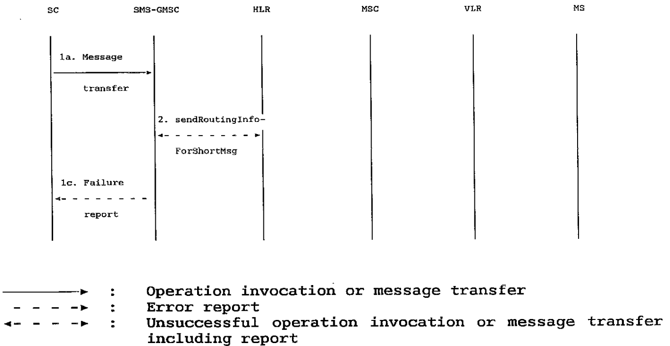
Figure 03.40/15 c). Short message transfer attempt failing due to negative outcome of HLR information retrieval.
